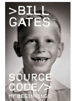
Source Code
